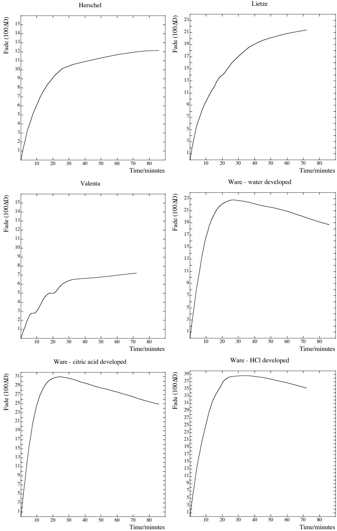
Fig. 9.3 Variation of fade with exposure time (at 4 kilolux)
