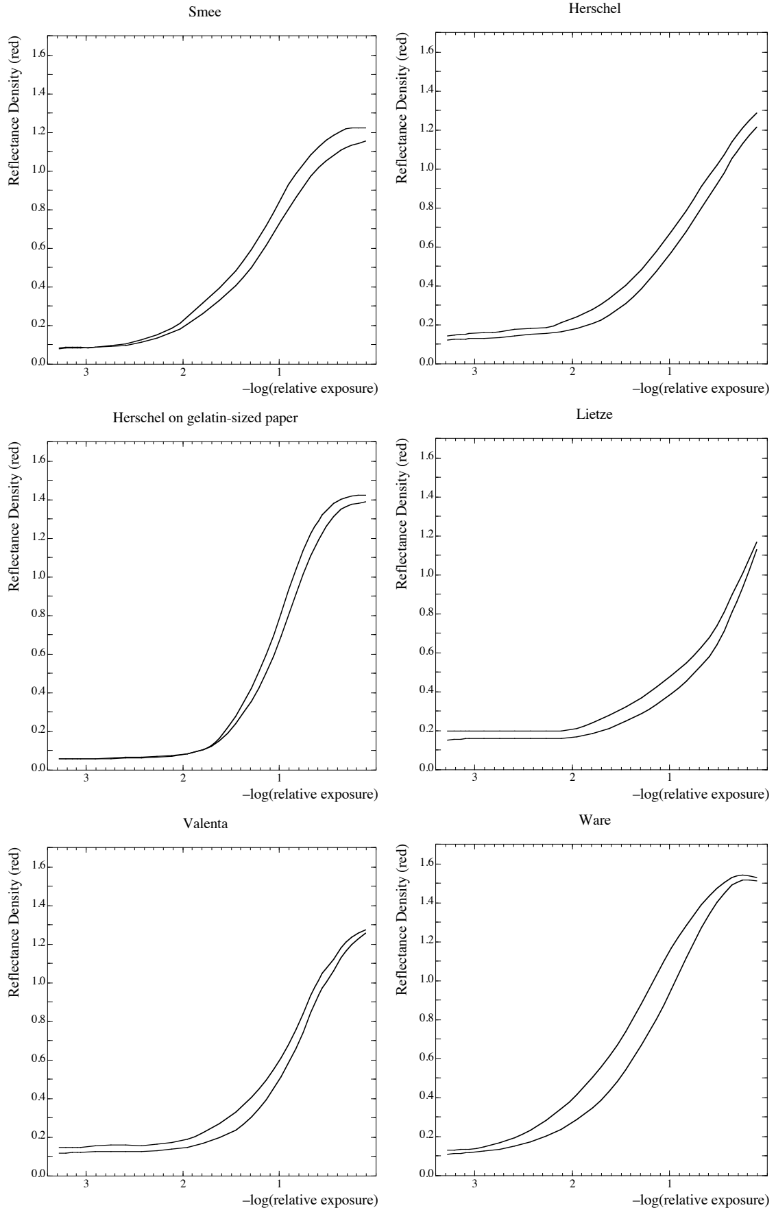
Fig. 9.1 Characteristic curves for cyanotype sensitizers
