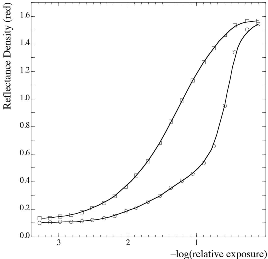
Fig. 7.1 Characteristic curve for New Cyanotype without dichromate. 1% acid developed (left) and water developed (right)
