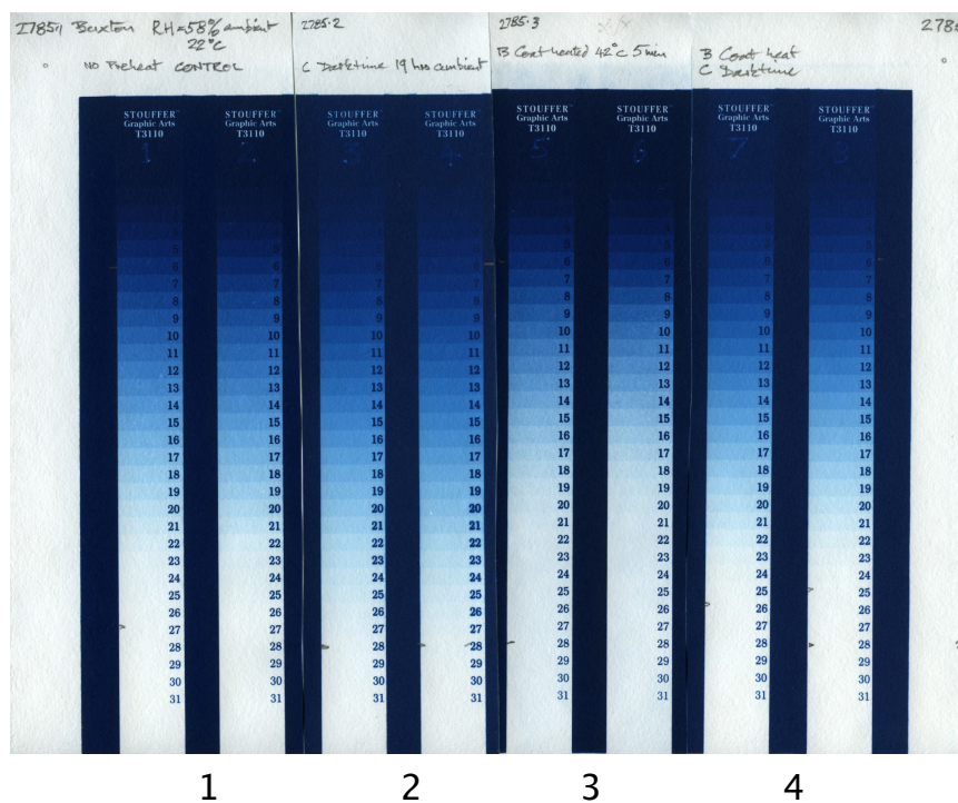
Fig 7.3 Effects of heat drying sensitizer and 'darktime' exposure 1 Control: no heat-dry or darktime; 2 Darktime only: 19 hours at 58% RH 3 Heat-dry only: 42°C for 5 mins; 4 Heat-dry and 19 hours darktime.
