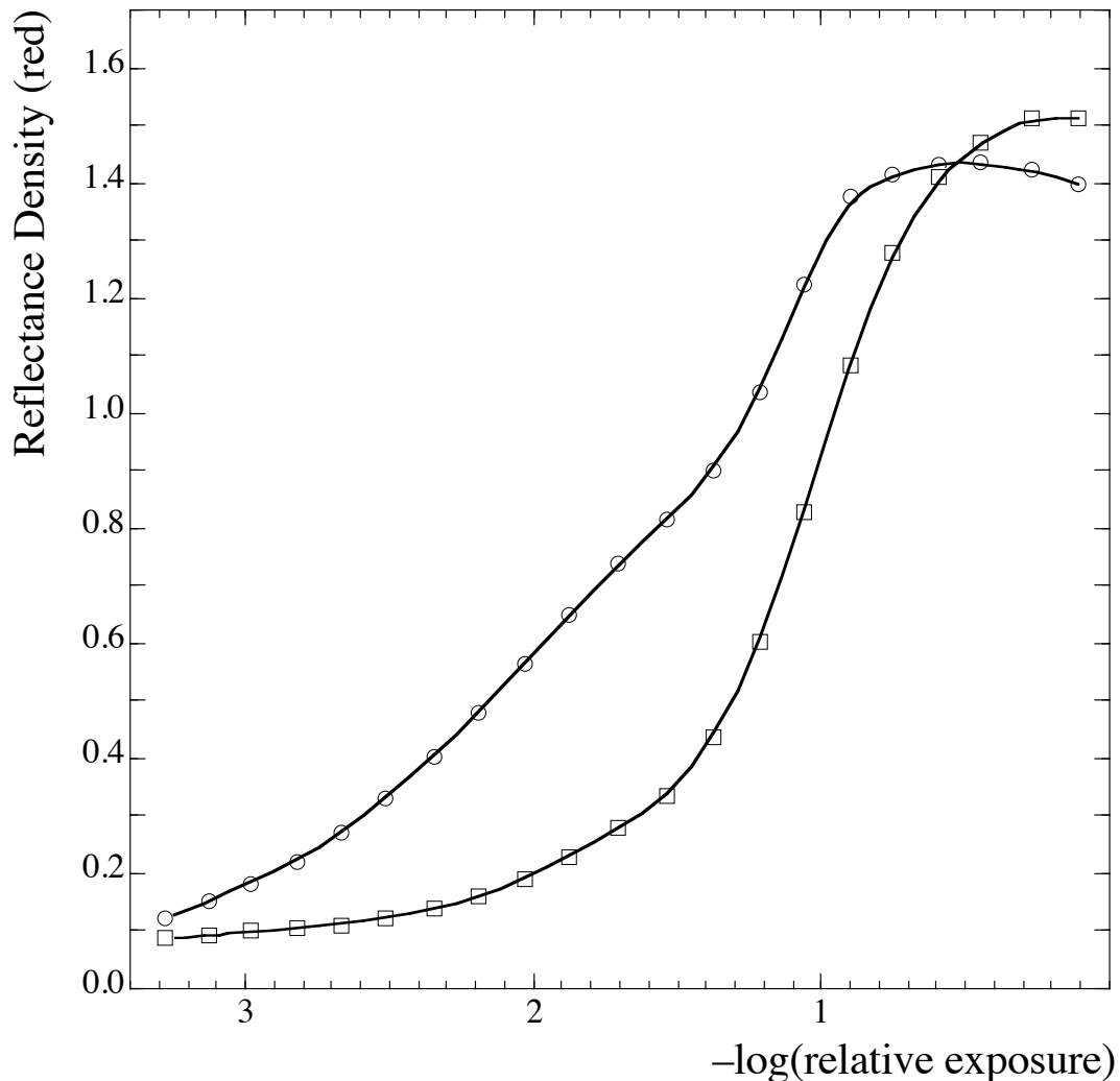
Fig. 7.2 Characteristic curve for New Cyanotype with 0.1% dichromate 1% acid developed (right) and water developed (left) 4x exposure
