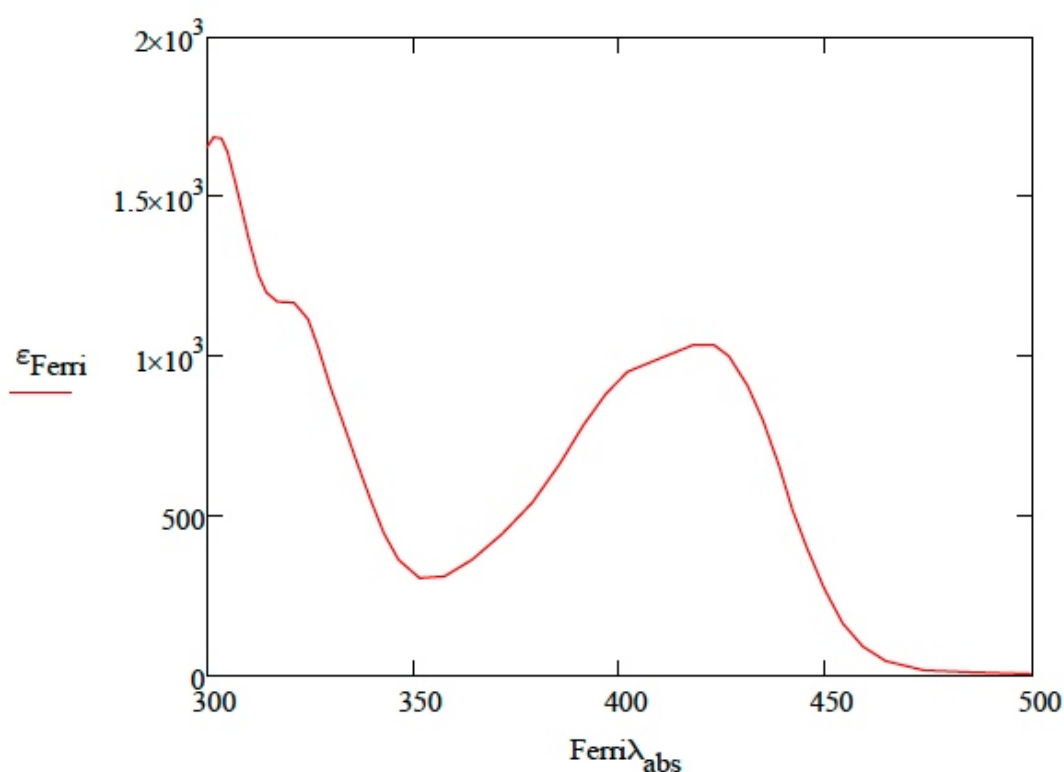
Fig. III.3 UV–Visible absorption spectrum of \text{Fe}(\text{CN})_6^{3-}
