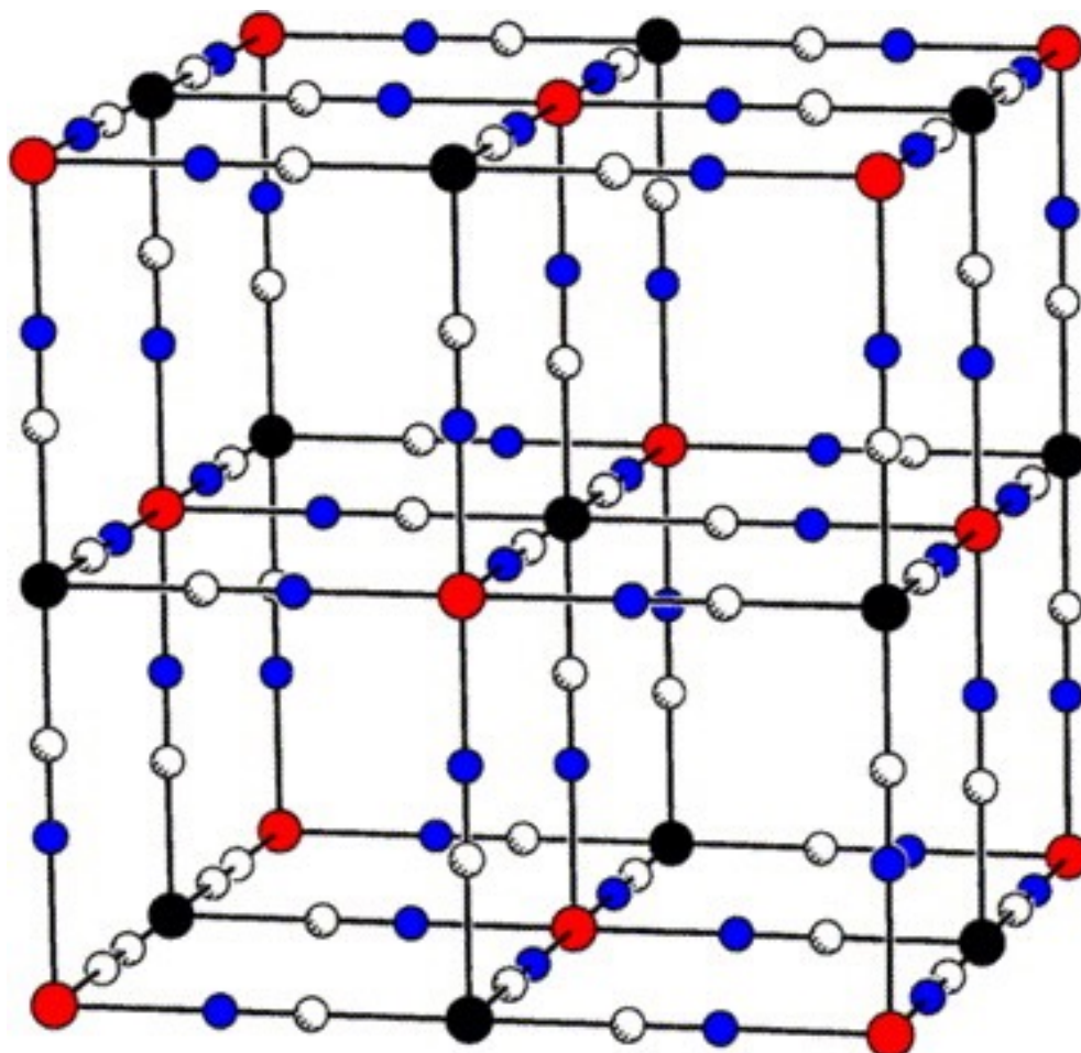
Fig. 3.2 The idealised crystal lattice of Prussian blue
