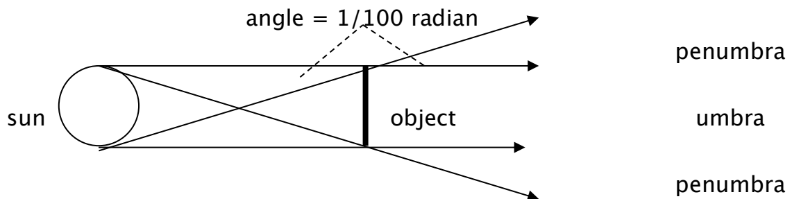
Fig 6.1 The structure of a solar shadow (not to scale).
