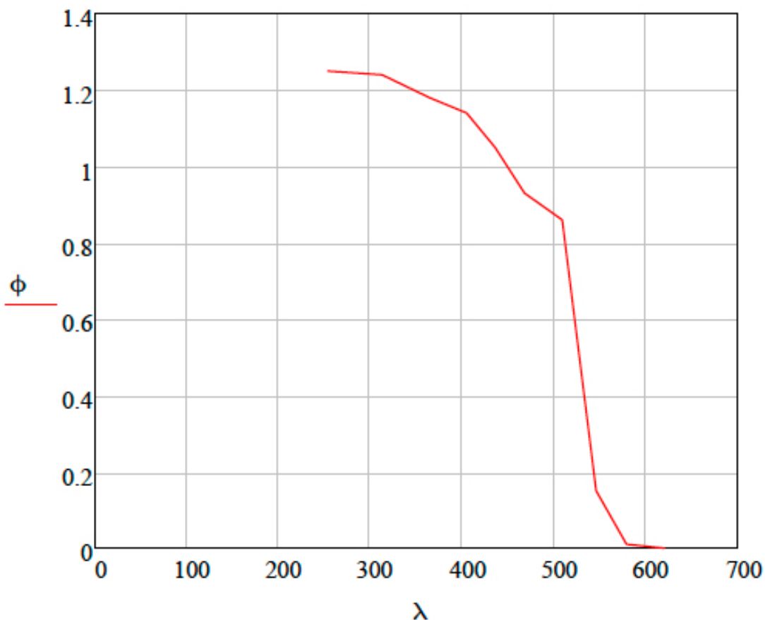
Fig. III.1 Quantum yield of \text{Fe}(\text{C}_2\text{O}_4)_3^{2-}
