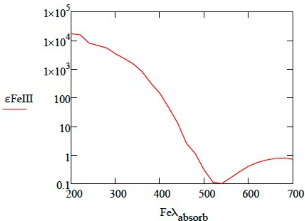
Fig. III.2 UV-Visible absorption spectrum of \text{Fe}(\text{C}_2\text{O}_4)_3^{2-}
