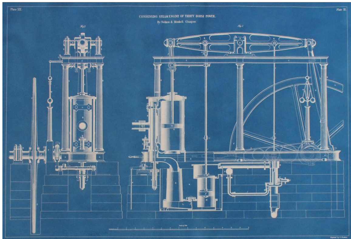
Fig. 1.5 Blueprint of a steam engine
