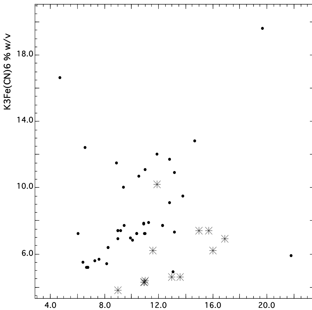
Ammonium ferric citrate % w/v * green salt; • brown salt Fig 4.1 Compositions of historical cyanotype sensitizers (% w/v in final mixed sensitizer)
